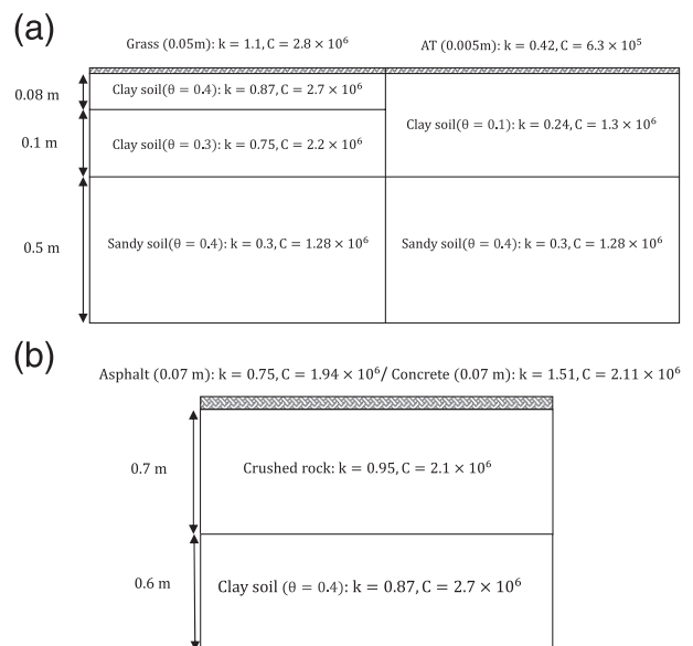
FIG. 3. (a) Subsurface layer depths and thermal properties for AT and grass surfaces; k is thermal conductivity ( \text{W m}^{-1} \text{K}^{-1} ), C is heat capacity ( \text{J m}^{-3} \text{K}^{-1} ), and \theta is volumetric water content. (b) Subsurface layer depths and thermal properties for asphalt and concrete surfaces; k , C , and \theta are defined as in (a).
