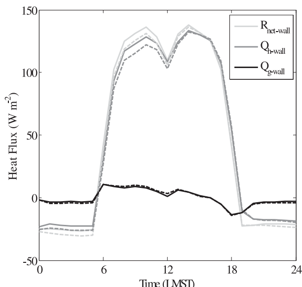
FIG. 7. Energy balance components averaged over the four walls for grass (solid line) and AT (dashed line); Q_{h\text{-wall}} is the wall-to-canopy sensible heat flux, Q_{g\text{-wall}} is the conduction heat flux into the wall, and R_{\text{net-wall}} is the net radiation on the building walls after multiple reflections. Area units refer to wall surface area.
