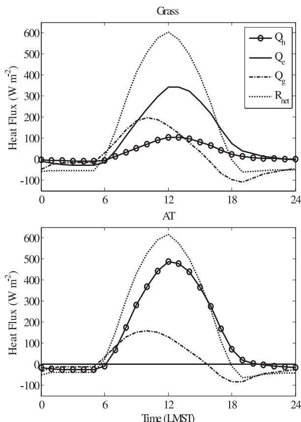
FIG. 6. Modeled energy balance components for the (top) grass and (bottom) AT surfaces; Q_h , Q_e , and Q_g are sensible, latent, and ground heat fluxes, respectively, and R_{\text{net}} is the net radiation.
